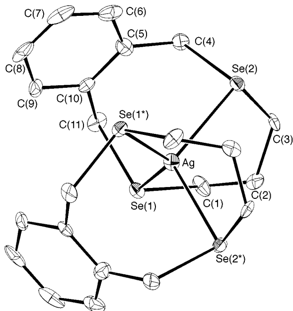
Fig. 4 View of the structure of [\text{Ag}(\text{L}^2)_2]^+ with the numbering scheme adopted. Atoms marked * are related by a crystallographic two-fold operation. Ellipsoids as in Fig. 1
