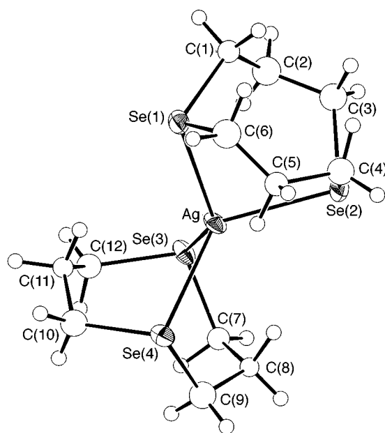
Fig. 3 View of the structure of [\text{Ag}(\text{L}^1)_2]^+ with the numbering scheme adopted. Ellipsoids as in Fig. 1
