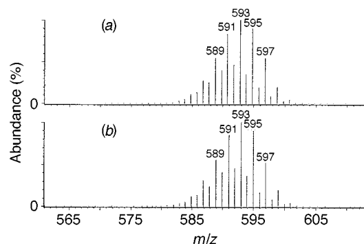
Fig. 5 Observed (a) and calculated (b) electrospray mass spectrum of [\text{Ag}([16]\text{aneSe}_4)]^+
